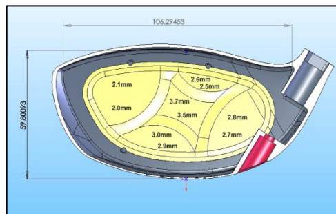
Advanced Multi-Level Face Design
