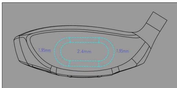
Variable Face Thickness for Max COR
