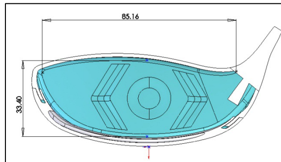
Boomerang Face Design
